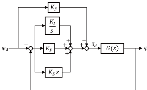
Fig. 4. Steering control system structure of bicycle
