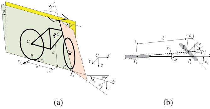
Fig. 1. (a) 3D sstructure of bicycle and (b) Top view of bicycle
