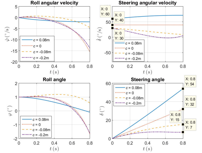
Fig. 3. bicycle dynamic characteristics simulation results
