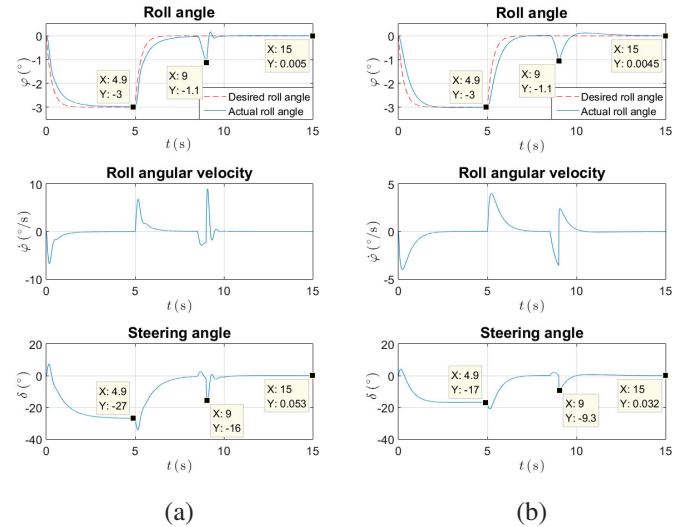
Fig. 5. Simulation results when (a) c = 0.08\text{m} , v_x = 1.3\text{m/s} and (b) c = -0.09\text{m} , v_x = 1.3\text{m/s}
