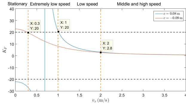
Fig. 7. The relationship between K_F and v_x under different trail length
