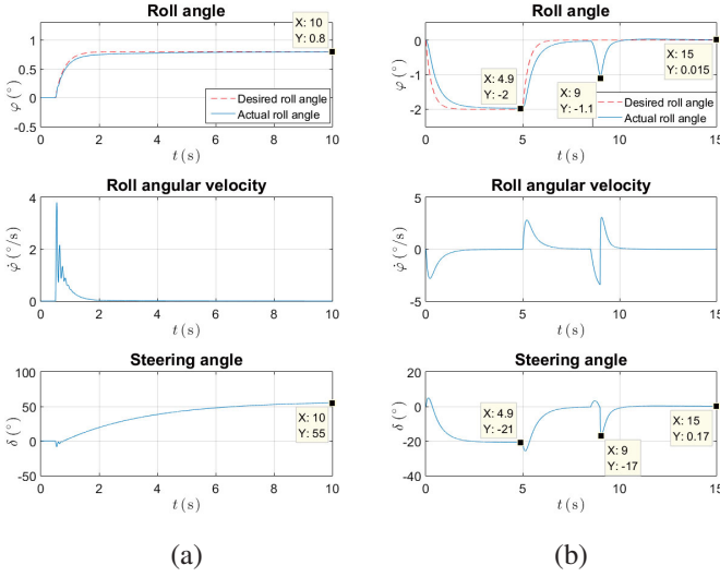
Fig. 6. Simulation results when (a) c = 0.08\text{m} , v_x = 0.8\text{m/s} and (b) c = -0.09\text{m} , v_x = 0.8\text{m/s}
