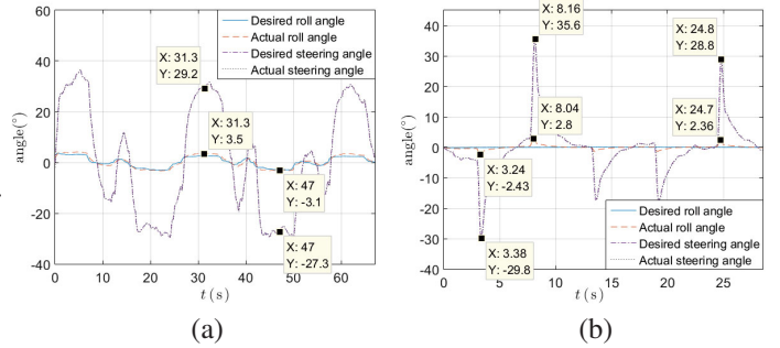
Fig. 9. (a) steering experiment result and (b) anti-interference experiment result when c = 0.08\text{m} , v_x = 1.3\text{m/s}
