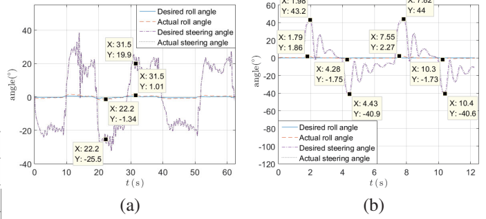
Fig. 11. c = -0.09\text{m} , v_x = 0.58\text{m/s} (a)steering experiment result and (b) anti-interference experiment result
