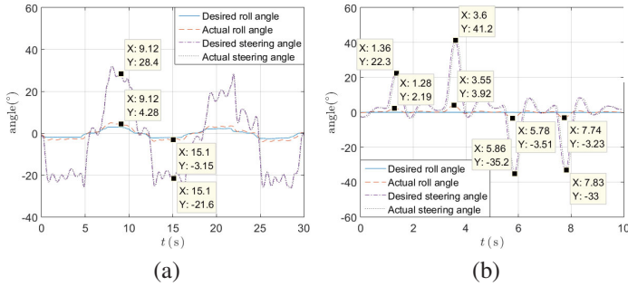
Fig. 10. (a)steering experiment result and (b) anti-interference experiment result when c = -0.09\text{m} , v_x = 1.3\text{m/s}
