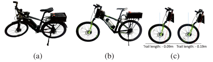
Fig. 8. (a) Bicycle Prototype 1, (b) Bicycle Prototype 2 and (c) different trail lengths of Prototype 2
